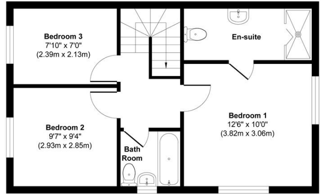
First Floor Approximate Floor Area 451 sq. ft (41.92 sq. m)
