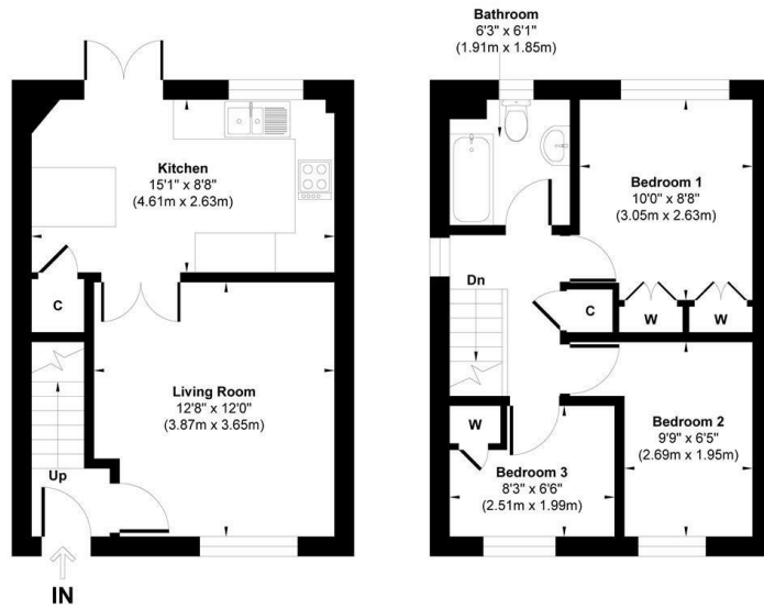
Ground Floor Approximate Floor Area 330 sq.ft (30.66 sq.m)
